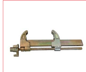
Master clamp, adjustable Adjustment range up to 20cm
