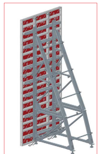
Brace frame "S" incl. attachable frame up to 6m
