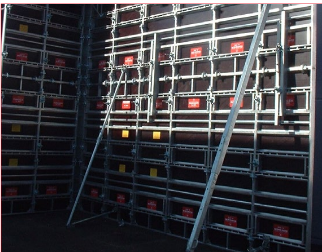
Push-pull prop and push-pull prop "G"
